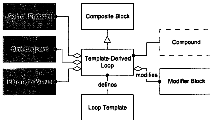
Figure 91 - Template-Derived Loop object model
